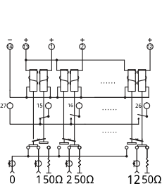
Latching
