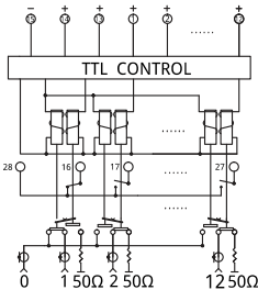
Latching & TTL
