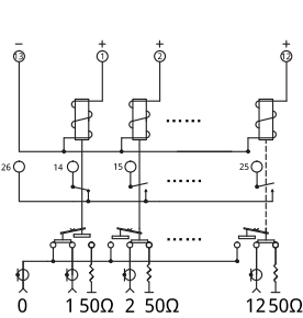
Normally Open
