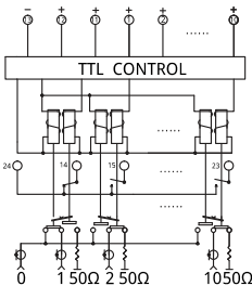
Latching & TTL
