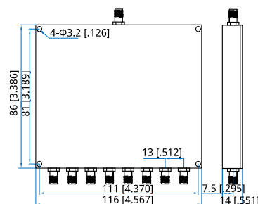
Outline A
