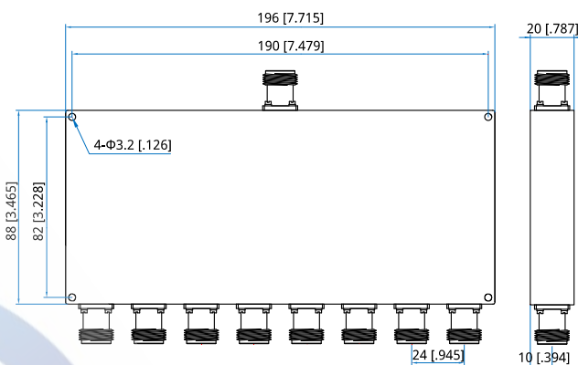
Outline B
